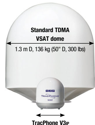
TracPhone V3IP 39.4 cm D, 11.3 kg (15.5" D, 25 lbs)
